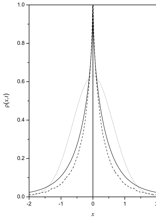
Fig. 1. Behavior of \rho(x, t) versus x is illustrated. The solid line corresponds the case \bar{D} = 1 and \mathcal{D}_\gamma = 1 , with \eta = -1/2 and \gamma = 2/3 , and the dashed line is the case \bar{D} = 0 and \mathcal{D}_\gamma = 2 , with \eta = -1/2 and \gamma = 2/3 . The dotted line is the usual case, i.e., \bar{D} = 1 and \mathcal{D}_\gamma = 1 , with \eta = 0 and \gamma = 1 . We also consider, for simplicity, the initial condition \rho(x, 0) = \delta(x) .
