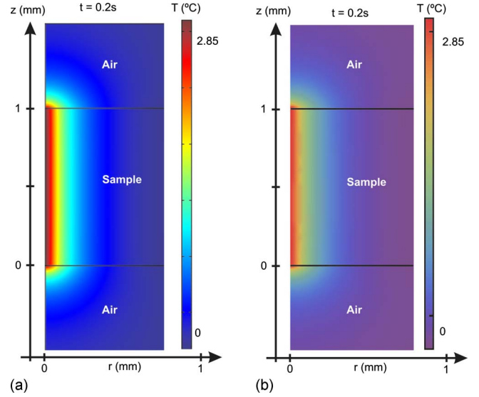
FIG. 6. (Color online) Density plot using (a) the FEA and (b) the analytical approximation models.
