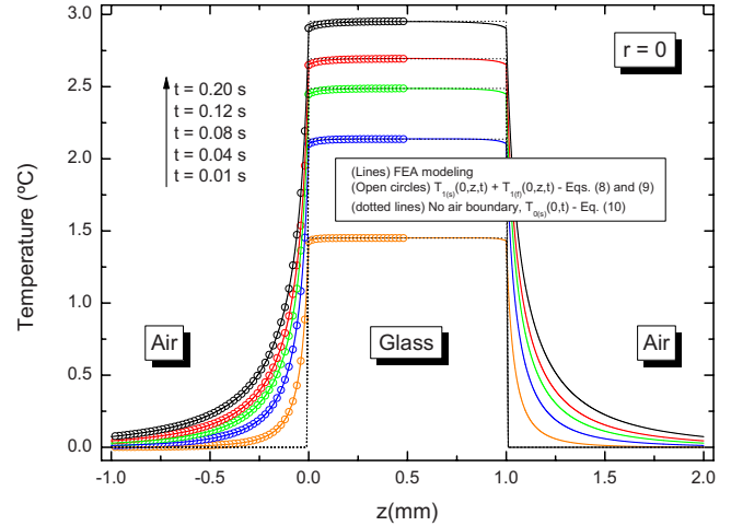
FIG. 3. (Color online) Temperature profile along the z direction (air-glass-air) using the FEA modeling, the solution considering air surroundings, Eqs. (8) and (9), and the solution with no transfer of heat from glass to air, Eq. (10), at different exposure times. r=0 was used in the simulations.
